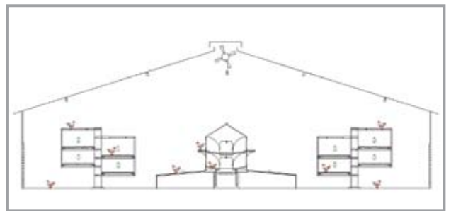
Combination design - with manure pit
